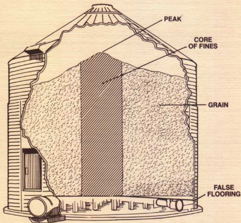
FIG. 4. With center filling of a grain bin, fines accumulate in the center, forming a spoutline. Unload the spoutline and level the grain for even airflow through the grain.
