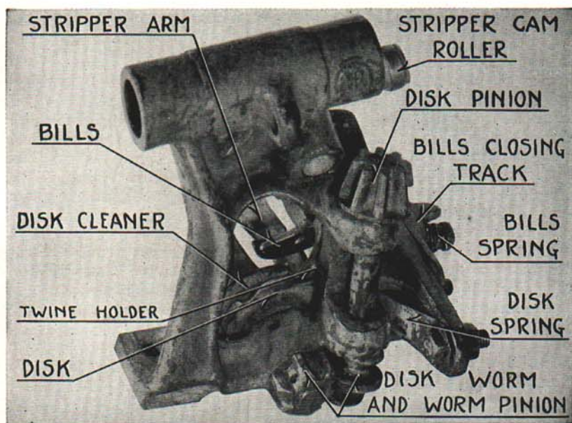
Fig. 12. Deering or I. H. C. Model D Knotter Head.
