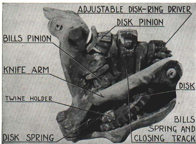
Fig. 14. Massey-Harris Knotter Head.
