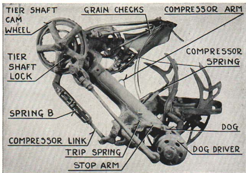
Fig. 2. Deere Binder Head.
