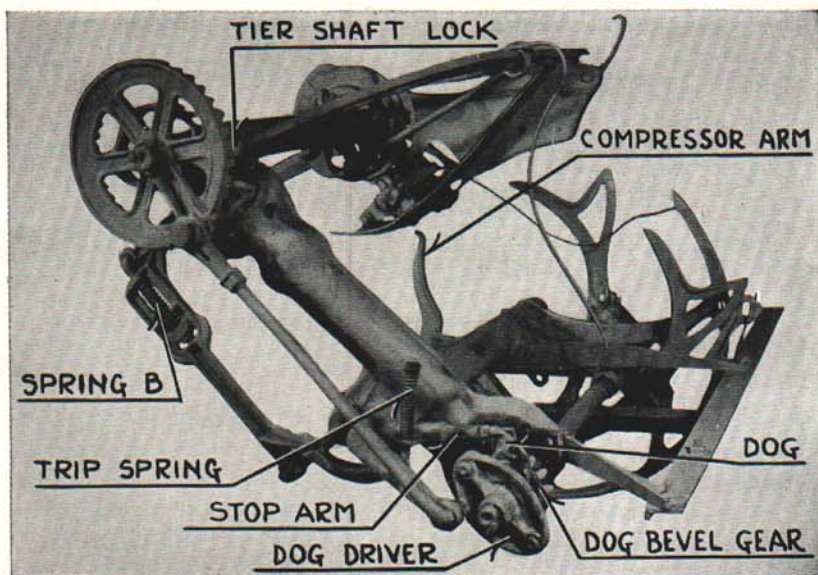
Fig. 1. Deering or I. H. C. Model D Binder Head.
