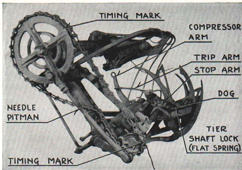
Fig. 4. Massey-Harris Binder Head.
