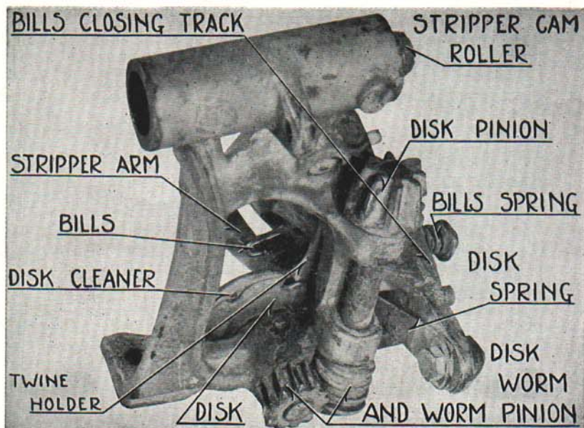
Fig. 13. Deere Knotter Head.
