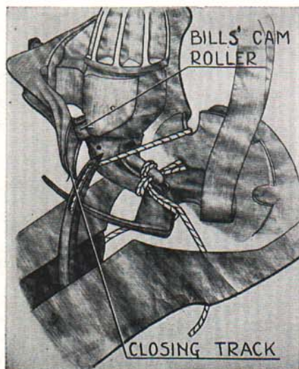
Fig. 10. Step 5 in the Tying Process.
