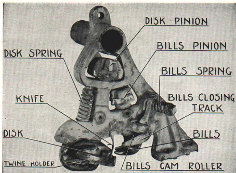
Fig. 11. McCormick or I. H. C. Model M Knotter Head.
