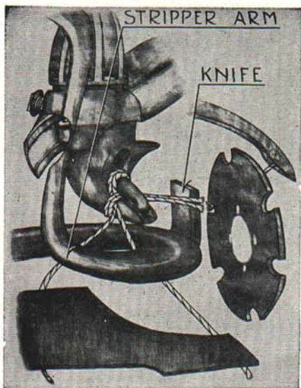
Fig. 9. Step 4 in the Tying Process.
