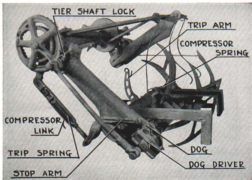
Fig. 3. McCormick or I. H. C. Model M Binder Head.
