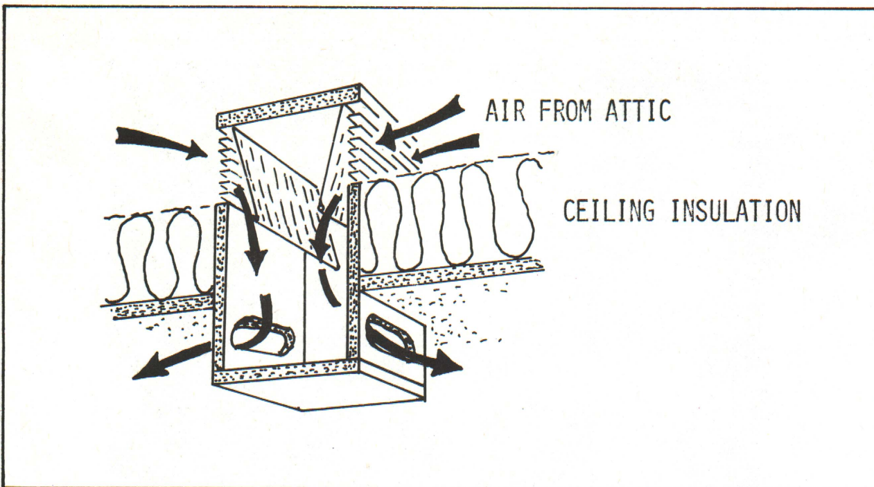
Figure 8. Rectangular ceiling area intake with self-adjusting damper.
