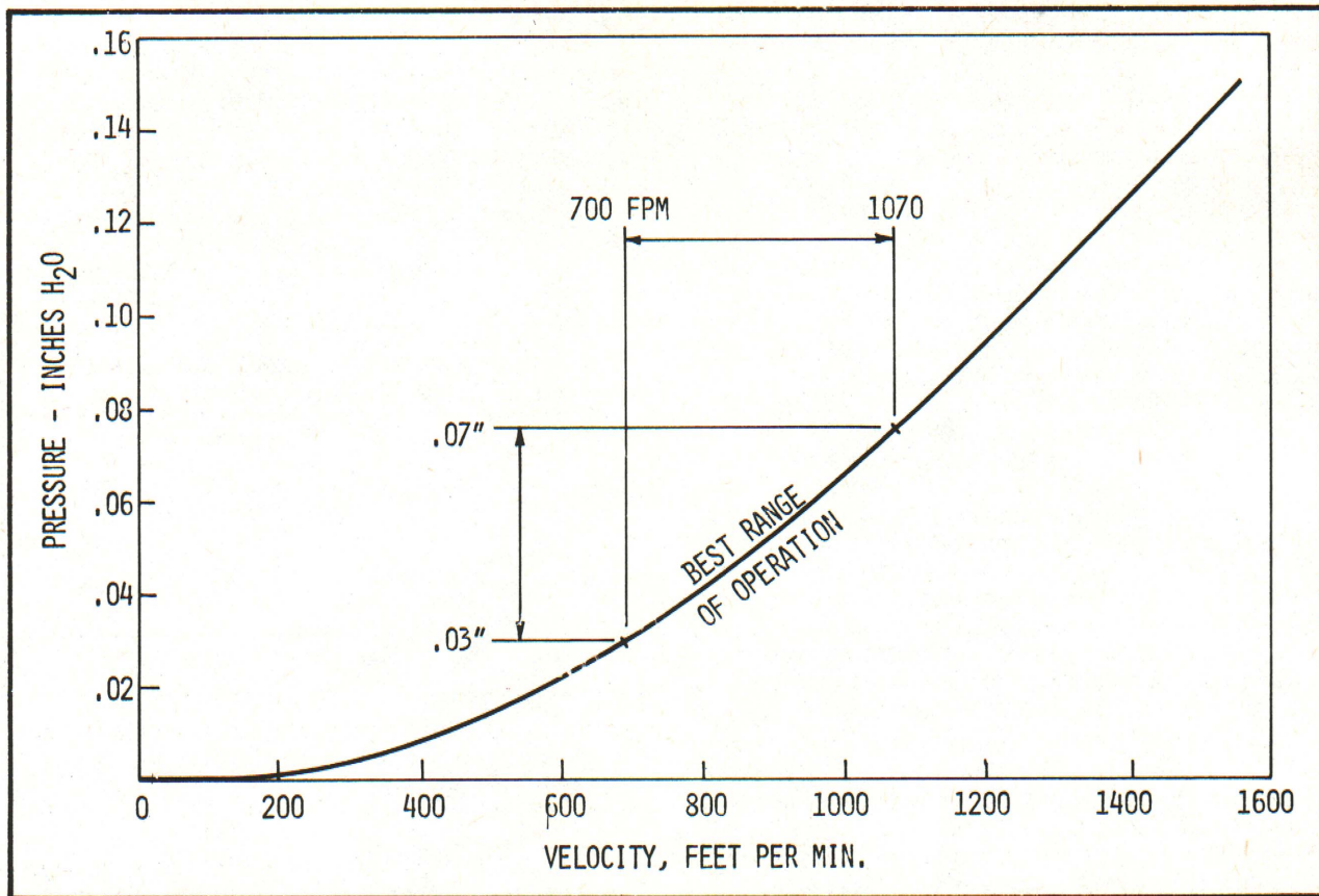
Figure 6. Air intake velocity and static pressure relationship.
