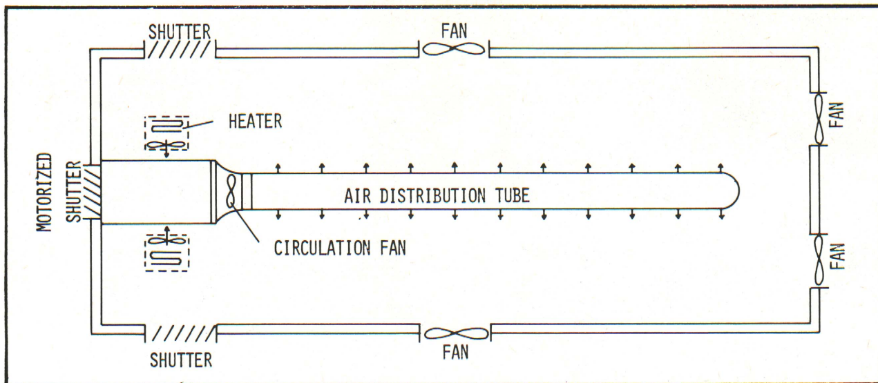
Figure 4. Positive pressure intake and air distribution.
