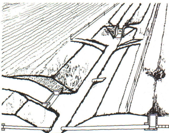
Figure 8. Suitable outlets for both surface and tile drains frequently require special structures which increase initial costs but lengthen the life of the ditch.
