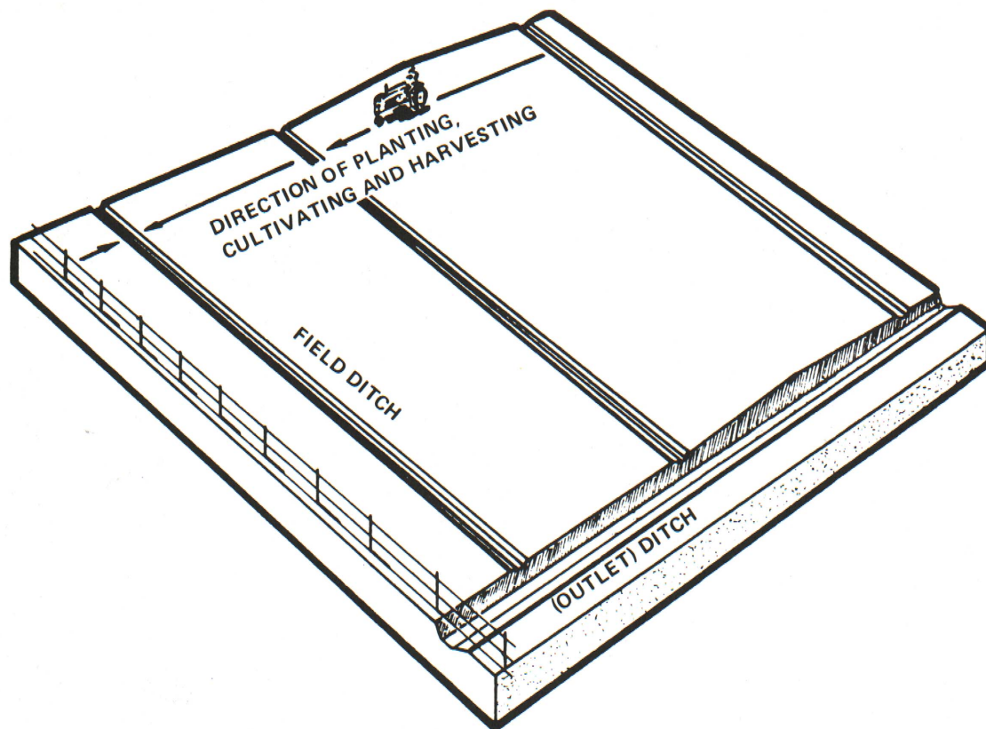
Figure 4. Parallel field ditches for surface drainage work well on nearly level fields. Spacings vary with kinds of soil and distance and amount of soil material to be moved. Make outlet ditches at least 1 foot deeper than field ditches. Grade to outlet ditch should be such that erosion does not occur.
