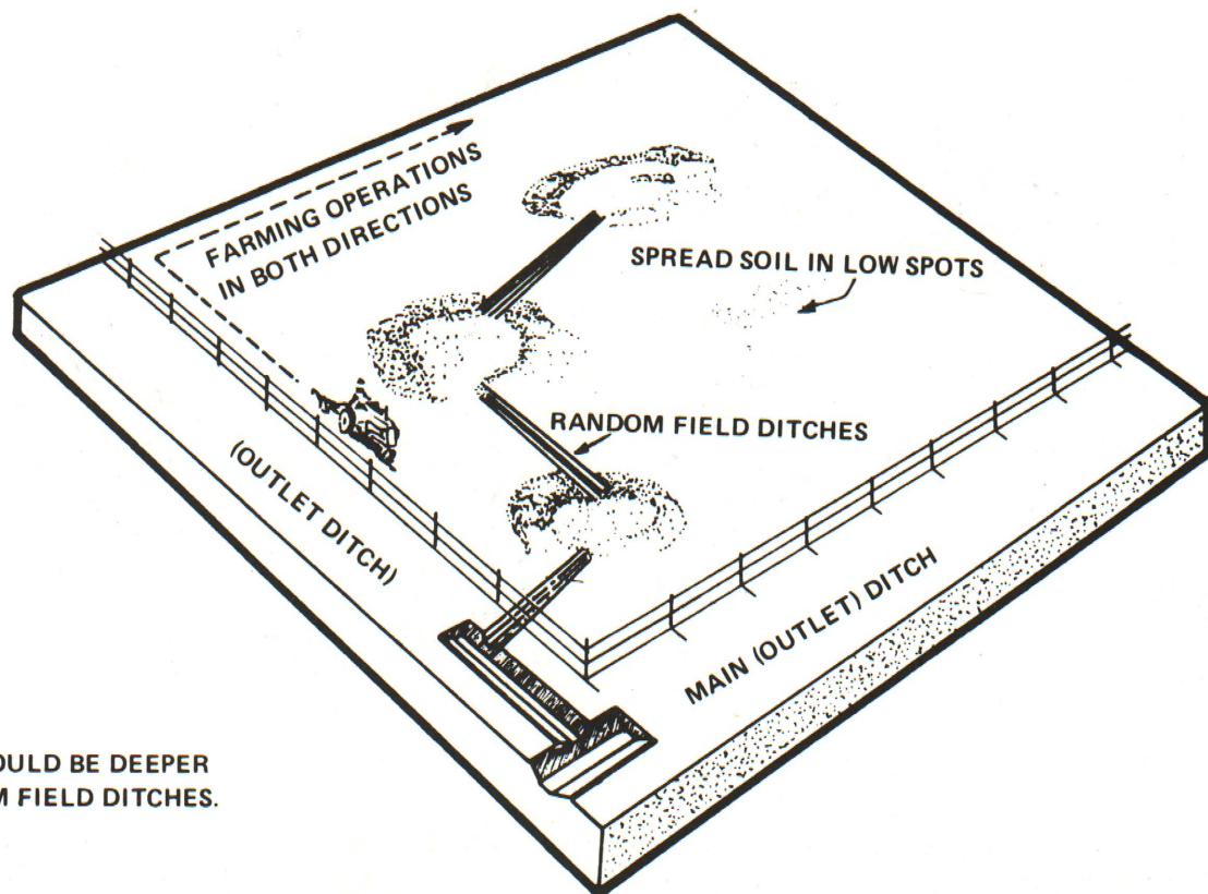
Figure 5. Random field ditches can improve crop yields in many parts of the state.
