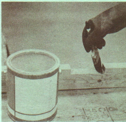
Fig. 17. When treated wood is cut, the sawed surfaces should be well brushed with preservative.
