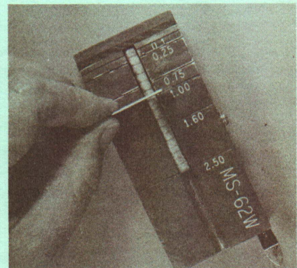
Fig. 10. Boring jigs like this are used for sectioning samples for analysis to determine amount of preservative in wood.
