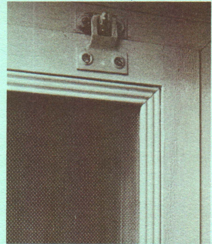
Fig. 5. Painting defects caused by excess absorption of preservative by screen sash.
