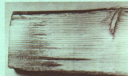
Fig. 11. A creosoted Douglas fir heartwood timber from a 25-yr-old bridge sawed open to reveal penetration of preservative. Side grain penetration is a fraction of end penetration but sufficient to protect a timber if no checks develop through the treated layer.
