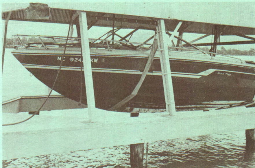
Fig. 6. This boat shelter made of CCA pressure-treated wood has been painted successfully for several years.
