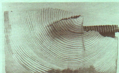
Fig. 7. Discolored wood from iron lag bolt in treated fir. This is a wood reaction not caused by preservative treatment.
