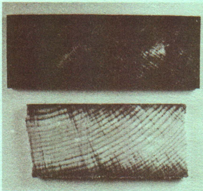
Fig. 12. Adequate and inadequate penetration in two ponderosa pine 2-in. planks cut at the center. A chemical indicator shows copper in CCA-treated wood.
