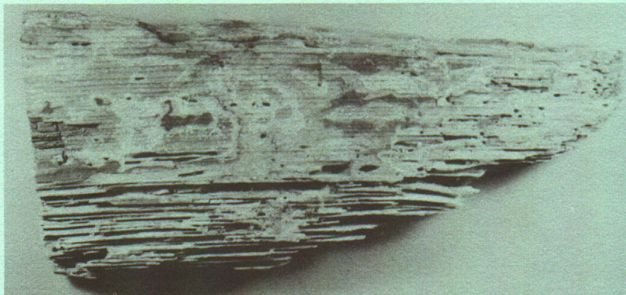
Fig. 12. (Left) Douglas fir plank damaged by termites. Note remaining harder summerwood and debris on surface and in excavated parts of wood. Fig. 13. (Right) Termite shelter tubes built over concrete block support under wood framed structure.
