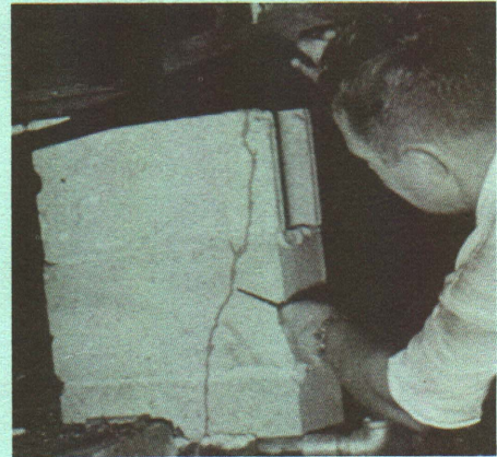
Fig. 12. (Left) Douglas fir plank damaged by termites. Note remaining harder summerwood and debris on surface and in excavated parts of wood. Fig. 13. (Right) Termite shelter tubes built over concrete block support under wood framed structure.
