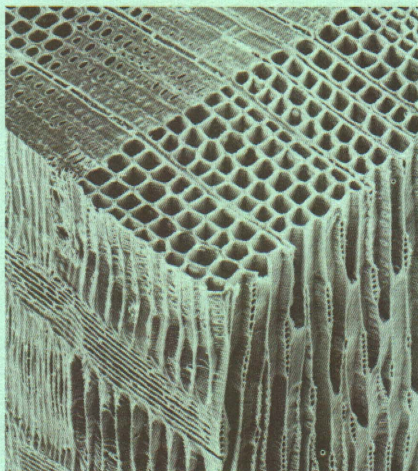
Fig. 2. Highly magnified (100X) view of a softwood. Note length of cells compared with width. Grain direction vertical. Summerwood cells with thick walls. (Photo courtesy N.C. Brown Center for Ultrastructure Studies at College of Environmental Science and Forestry, SUNY.)
