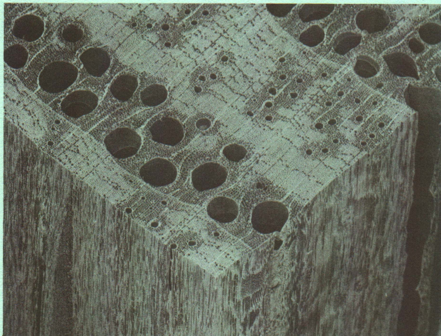
Red oak, highly magnified, a hardwood with a variety of cell types. (N.C. Brown Center for Ultrastructure Studies, College of Environmental Science and Forestry, SUNY)
