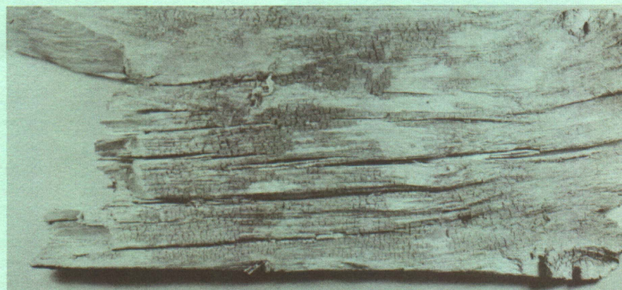
Fig. 8. Board surface destroyed by soft rot. Note small cross checks.
