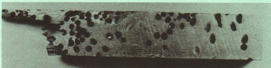
Fig. 18. Shipworm damaged wood cut from rafted logs.
