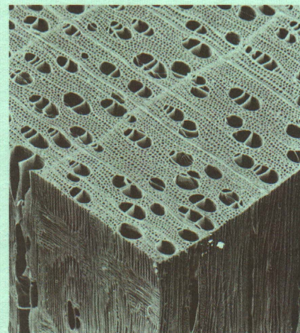
Fig. 3. Hardwood highly magnified. Greater variety of cells than in softwood. Large cells are water-conducting vessels. (From Core, Côte and Day, Wood-Structure and Identification, by permission Syracuse University Press.)
