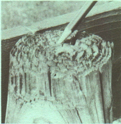
Fig. 9. Springwood portion of treated post eroded by soft rot.
