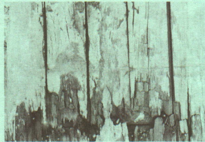
Fig. 5. (Left) Fruiting body resembling a mushroom growing from wood that appears sound on the surface but is decayed within. Fig. 6. (Center) Deck boards decayed by brown rot. Fig. 7. (Right) White rotted wood.
