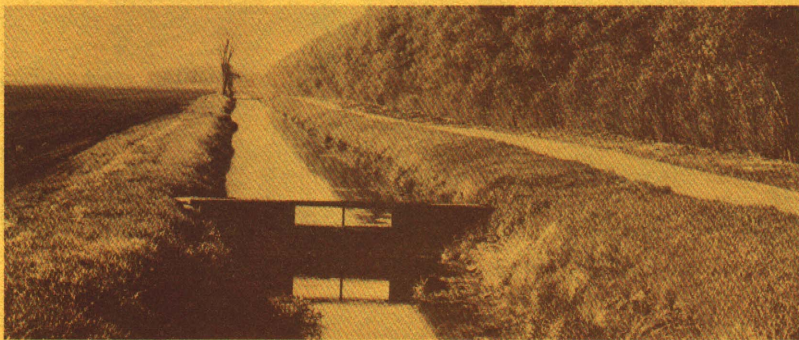
Fig. 3. Dams in ditches help regulate water table depths. High water tables should be maintained during winter months and in spring until field work starts.
