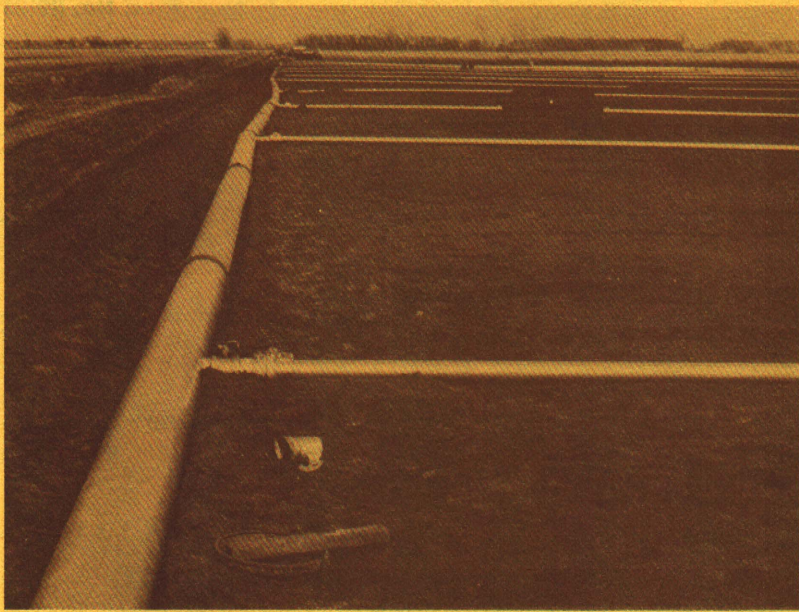
Fig. 2. Installing solid set irrigation pipe after planting carrots to reduce soil losses. Water should be applied before the surface soil dries and before the wind blows.
