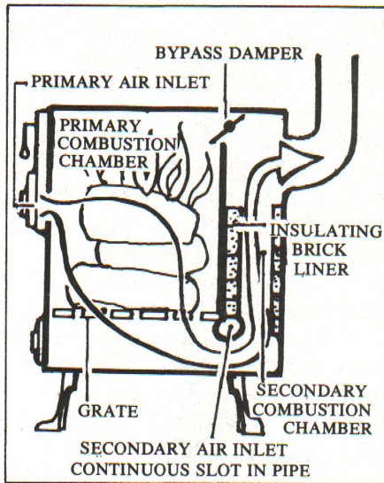
The stove has a secondary air inlet and a secondary combustion chamber.
