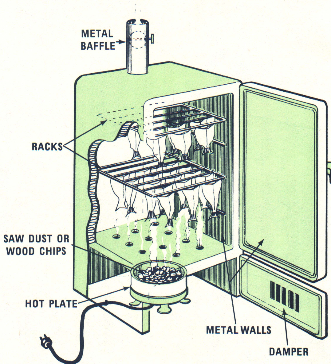
Smokehouse made from converted refrigerator. Note metal walls.
