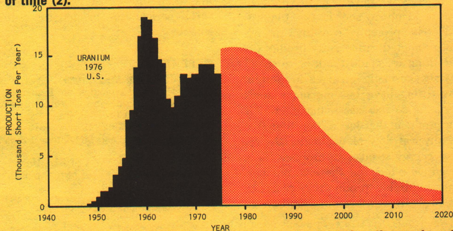
Figure 6—Cumulative production of uranium and cumulative discoveries of uranium as a function of time (3).
