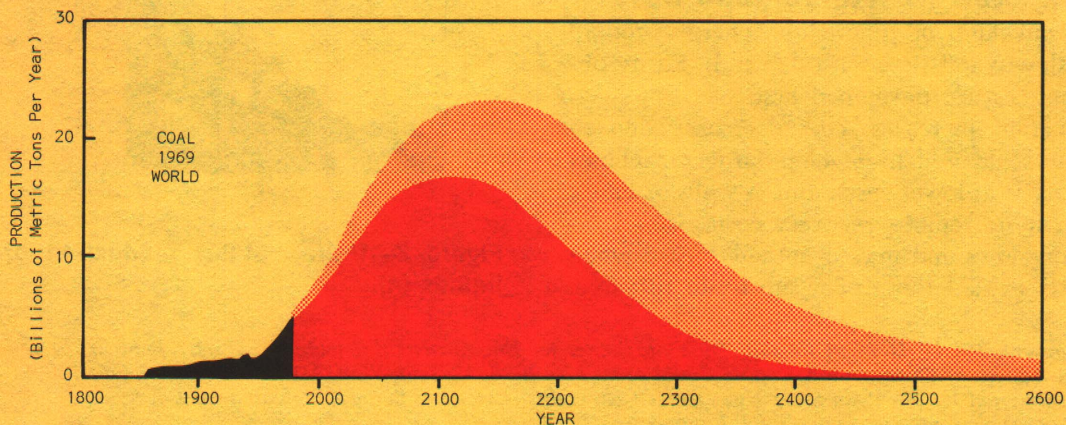
Figure 4—Complete cycle of United States coal production for two estimates of total supply (1).
