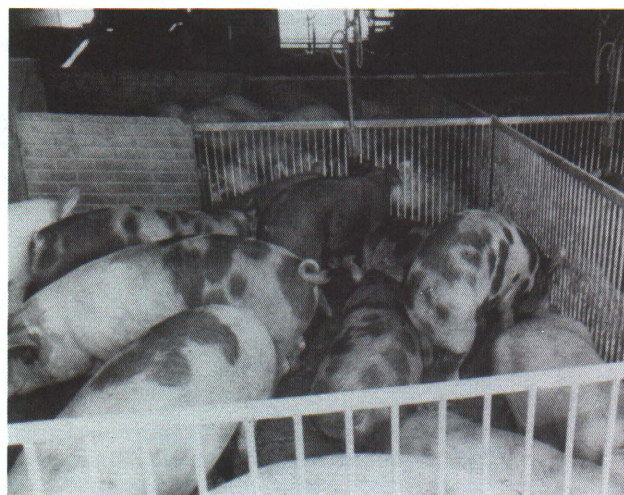
Figure 4. Cast-in-place concrete partitions (decorative form shown here) on the solid portion of the floor with vertical bar gates over the slats.
