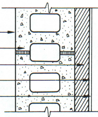
Figure 1. Insulated masonry wall. Omitting polystyrene foam insulation would reduce insulation R value to less than 3. This masonry block wall with only cores filled with vermiculite provides a total R of less than 6.
