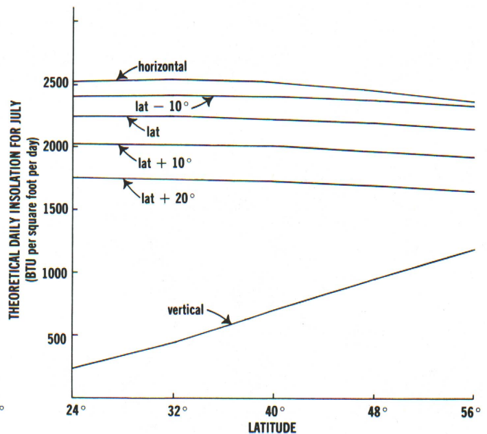
Figure 5. July insolation for several collector orientations and latitudes (1).
