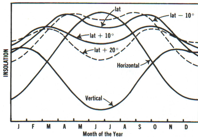
Figure 3. Differences between flat plate collector orientations and amount of solar radiation that can be captured (6).
