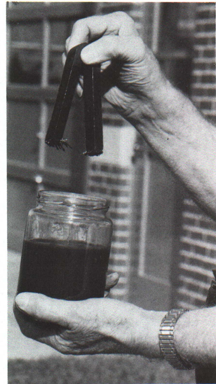
Fig. 2 — There may be a serious problem if a magnet pulls metal chips and particles from a sample of transmission lubricant.
