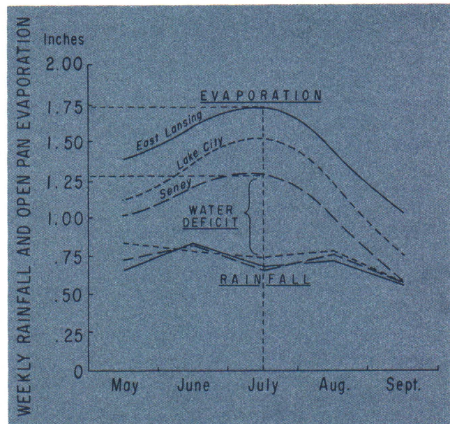
Figure 1. Weekly rainfall and open pan evaporation throughout the growing season for three locations in Michigan (Data from Nurnberger, Fred V., 1976 Summary of Evaporation in Michigan, M.D.A., Michigan Weather Service, 1407 S. Harrison Road, E. Lansing, MI).
