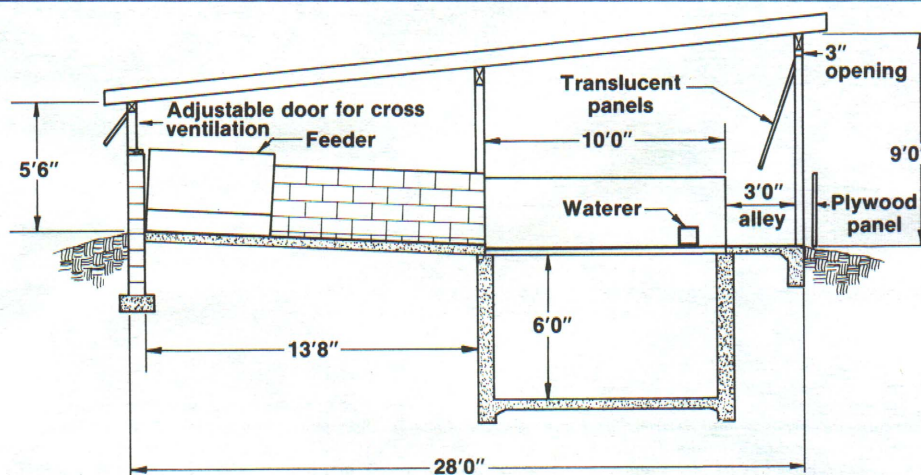
Figure 4. Modified open front, single slope roof.
