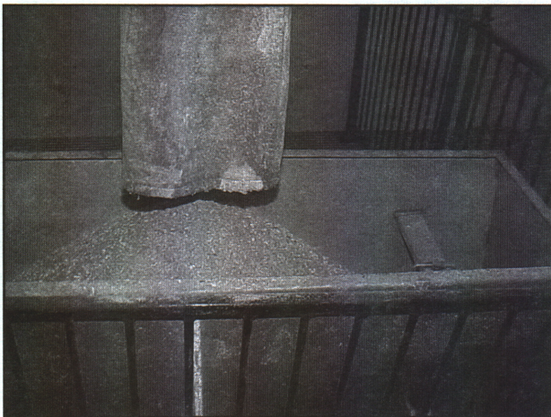
Figure 2. Placing covers over feed drop spouts can reduce dust.
