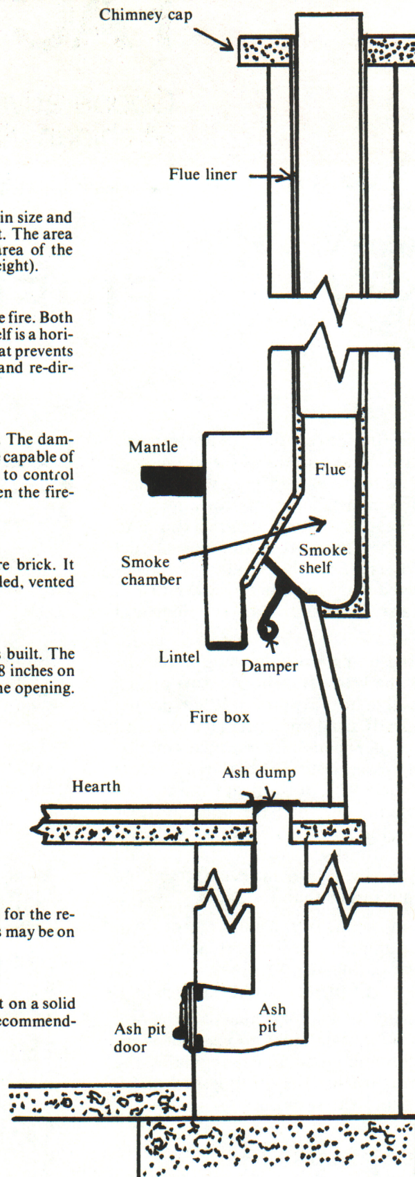
Fig. 3. Fireplace cross section.
